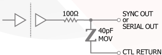
Figure 24: Internal circuitry for SYNC OUT and SERIAL OUT pins.
